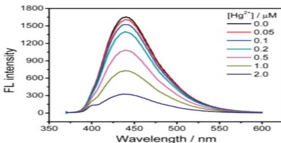
Figure 3. Effects of different concentrations of \text{Hg}^{2+} on the fluorescence of silicon nanoparticles.
